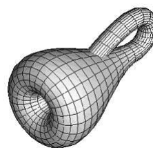
Klein bottle
